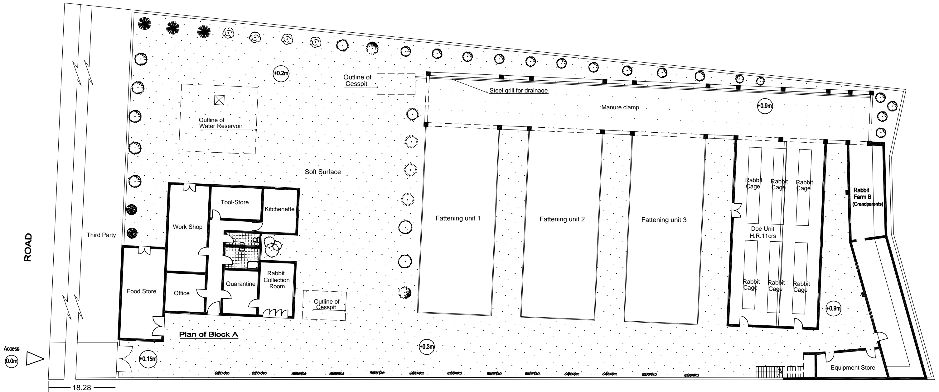
Proposed Block Plan
